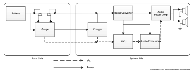
Wireless (Bluetooth) Speaker Application Block Diagram
